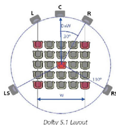
Dolby 5.1 Layout
